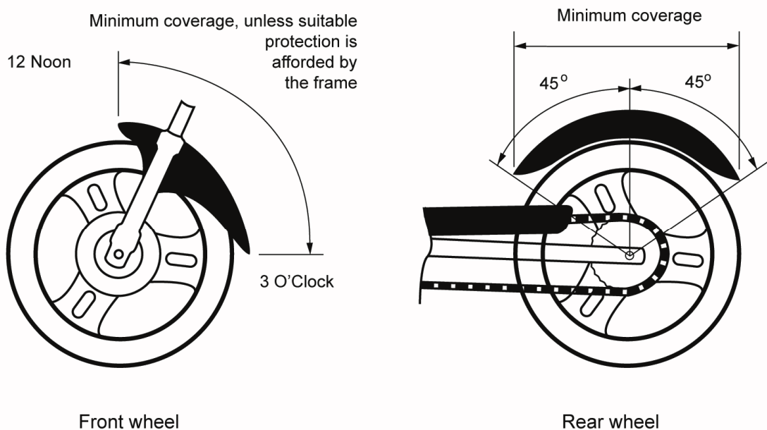
Figure LL2 Mudguard dimensions
